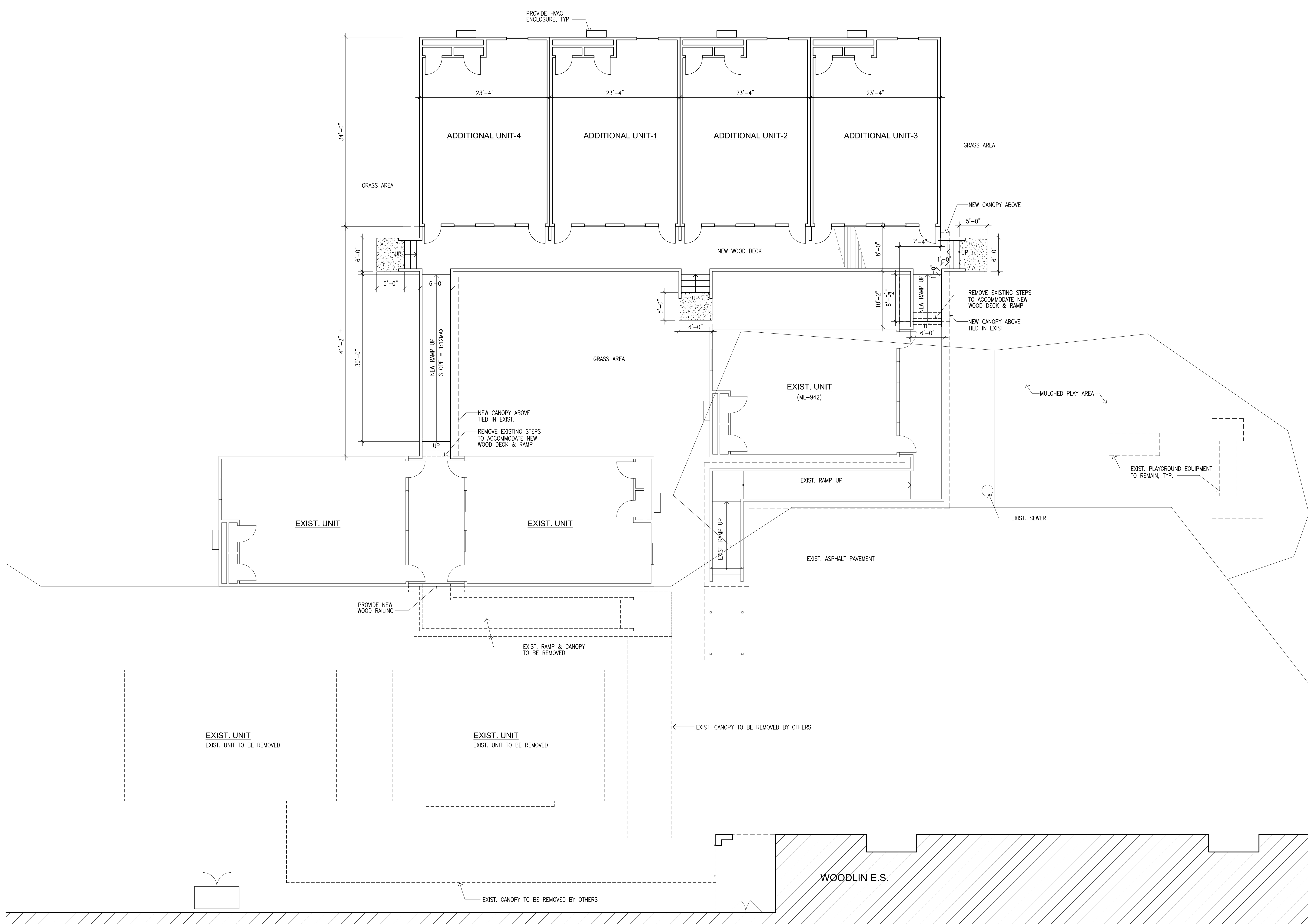
1 A-1 PROPOSED FLOOR PLAN SCALE: 1/8"=1'-0"
